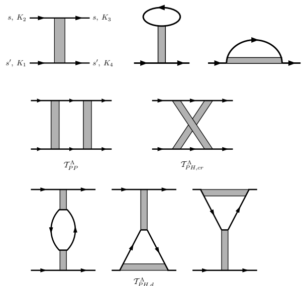
FIG. 8 Top row: The coupling function V^\Lambda(K_1, K_2, K_3) with the spin convention, and the diagrams entering in the flow equation for the self-energy (middle and right diagram). Middle and bottom row: The diagrams for the flow of the coupling function. The internal lines are either full propagators G^\Lambda or single-scale propagators S^\Lambda .
