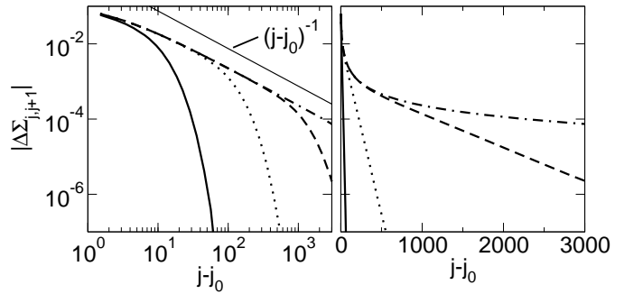
FIG. 19 Decay of the oscillatory part of the off-diagonal matrix element of the self-energy away from a single hopping impurity at bond j_0, j_0 + 1 . Results for t' = 0.1 , j_0 = 5000 , N = 10^4 , U = 1 , n = 1/2 , and different temperatures T = 10^{-1} (solid line), T = 10^{-2} (dotted line), T = 10^{-3} (dashed line), and T = 10^{-4} (dashed-dotted line) are presented. The left panel shows the data on a log-log scale, the right panel on a linear-log scale. For comparison the left panel contains a power-law (j - j_0)^{-1} (thin solid line) (Enss et al. , 2005).
