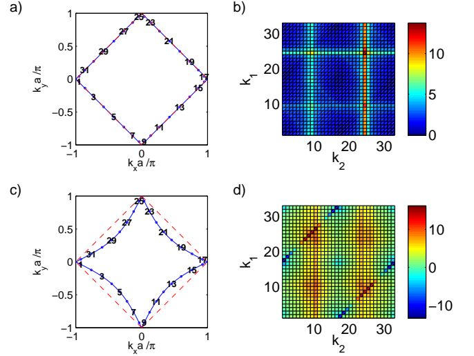
FIG. 10 (Color online) N -patch functional RG data obtained with the momentum-shell functional RG for the repulsive Hubbard model on the 2D square lattice. Upper plots: \mu = 0 , t' = 0 and initial U = 2t , lower plots: \mu = 1.2t , t' = -0.3t , U = 3t . To the left: Fermi surfaces for the two cases and the N = 32 discretization points for the two incoming \mathbf{k}_1, \mathbf{k}_2 and the 1st outgoing wavevector \mathbf{k}_3 . To the right: the coupling function V^{\Lambda*}(\kappa_1, \kappa_2, \kappa_3) with \kappa_3 = 1 and \kappa_1 and \kappa_2 moving around the Fermi surface. The colorbars on the right indicate the values of the interactions.
