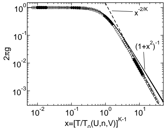
FIG. 20 One-parameter scaling plot of the conductance. Open symbols represent results obtained for U = 0.5 , n = 1/2 , and different T and V , while filled symbols were calculated for U = 0.851 , n = 1/4 . Both pairs of U and n lead to the same K = 0.85 (within the present approximation). The solid line indicates the non-interacting scaling function (1+x^2)^{-1} and the dashed one the LSG model power-law decay with exponent -2/K . (Data taken from Enss et al. (2005).)
