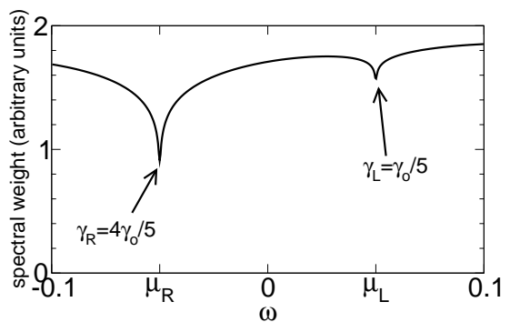
FIG. 26 Suppression of the local one-particle spectral weight as a function of energy near the left contact (at site 5) of an interacting wire driven out of equilibrium by a finite bias current. The parameters are T = 10^{-4} , N = 2^4 , U = 0.5 , t_L = 0.075 , t_R = 0.15 , and \mu_{L/R} = \pm 0.05 . (Data taken from Jakobs et al. (2007a).)
