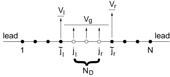
FIG. 17 Schematic plot of the quantum dot situation, where the barriers are modeled by two site impurities (Enss et al. , 2005).
