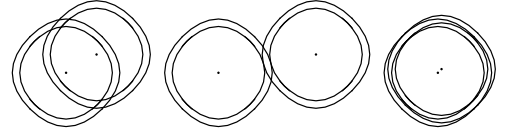
FIG. 28 Intersections of a momentum shell around the Fermi surface with its translate, as arising in loop integrals on the right hand side of the RG equation. When the Fermi surface is curved, the intersection volume decreases strongly unless the translating momentum is small.
