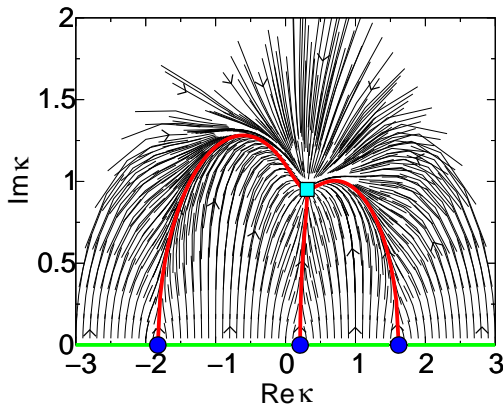
FIG. 24 (Color online) Flow of \kappa for U = -1 , n = 1/2 , and \phi = 0.4\pi . Arrows indicate the direction for U < 0 . For U > 0 it is reversed. For details see the text (Barnabé-Thériault et al. , 2005).
