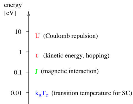
FIG. 1 (Color online) Important energy scales in high-temperature superconductors of the cuprate family. Magnetic interactions and superconductivity are generated from the kinetic energy (hopping) and the Coulomb repulsion.
