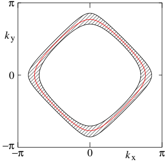
FIG. 2 (Color online) Momentum space region around the Fermi surface excluded by a sharp momentum cutoff for fermions with a tight-binding dispersion on a two-dimensional square lattice (lattice constant = one).
