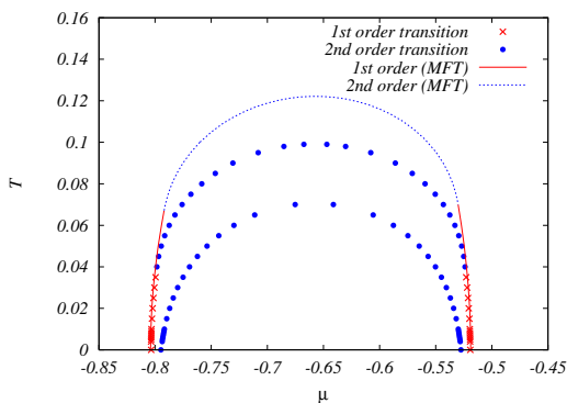
FIG. 16 (Color online) Critical temperatures versus chemical potential for \Lambda_0 = e^{-1} (larger dome with dots and crosses) and \Lambda_0 = 1 (smaller dome with dots). The mean-field transition line is also shown for comparison (Jakubczyk et al. , 2009).
