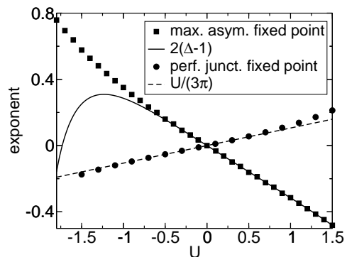
FIG. 25 Scaling exponents of the Y-junction close to the fixed points (Barnabé-Thériault et al. , 2005).
