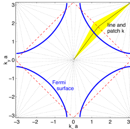
FIG. 9 (Color online) N -patch discretization of the Brillouin zone for the one-band Hubbard model on the 2D square lattice. The colored region is a patch in which the coupling function is approximated as a constant.
