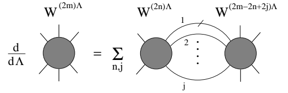
FIG. 27 Diagrammatic representation of the flow equations for the effective m -particle interactions W^{(2m)\Lambda} in the Wick-ordered version of the functional RG; the internal line with a dash corresponds to \partial_\Lambda \bar{G}_0^\Lambda , the others to \bar{G}_0^\Lambda ; all possible pairings leaving m ingoing and m outgoing external legs have to be summed.
