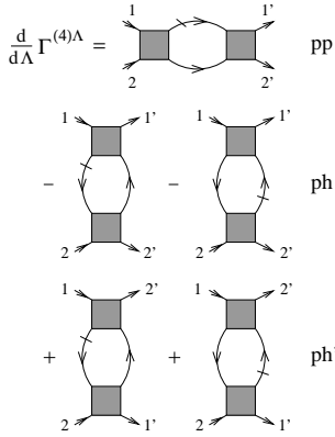
FIG. 4 Contributions to the flow of the two-particle vertex with particle-particle and particle-hole channels written explicitly, without the contribution from \Gamma^{(6)\Lambda} .
