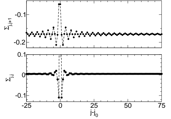
FIG. 18 Self-energy near a site impurity of strength V = 1.5 filling n = 1/4 , and interaction U = 1 ; the impurity is located at j_0 = 513 with N = 1025 sites. (Data taken from Andergassen et al. (2004).)
