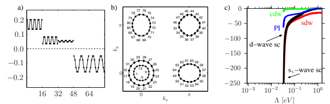
FIG. 12 (Color online) Functional renormalization group results for the iron pnictide compound LaFeAsO at moderate hole doping. a) Superconducting form factor as the outcome of functional RG, plotted versus the position on the hole pockets at \Gamma and M and electron pockets at X , numbered as depicted in b). The competing fluctuations manifest themselves in diverging ordering susceptibilities at low RG scales as shown in c), including in particular spin density wave (SDW), superconductivity (SC), Pomeranchuk (PI) and charge density wave (CDW) instabilities (Thomale et al. , 2011a).
