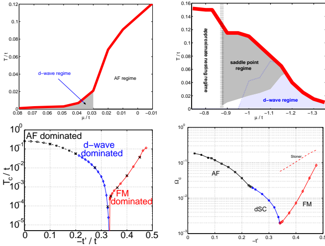
FIG. 11 (Color online) Leading instabilities as found by N -patch functional RG in the t - t' -Hubbard model. Left upper plot: T_* vs. \mu for band filling larger than unity, at t' = -0.3t and U = 3t . There is a high-energy-scale AF SDW instability with a weaker d_{x^2-y^2} -wave pairing instability when the AF-SDW is cut off. Data from Honerkamp (2001). Right upper plot: Data for the same t' and U on the 'hole-doped' side with band fillings smaller than one, from Honerkamp et al. (2001). Now there is a broad crossover 'saddle point regime' between the nesting-driven AF-SDW instability and the d_{x^2-y^2} -wave pairing regime. Lower left plot: T_* vs. t' at Van Hove filling where the Fermi surface contains the points (\pi, 0) and (0, \pi) . For large t' one finds a ferromagnetic instability. Data from Honerkamp and Salmhofer (2001a,b) obtained with the T -flow. Right lower plot: \Omega_* vs. t' at Van Hove filling, now obtained with the simplified vertex parametrization of Husemann and Salmhofer (2009) and with a soft frequency regulator \Omega .
