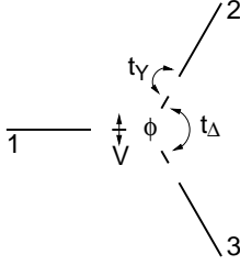
FIG. 22 Sketch of the symmetric Y-junction of three quantum wires (Barnabé-Thériault et al. , 2005).
