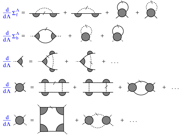
FIG. 7 Diagrammatic representation of the flow equations for the (fermionic and bosonic) self-energies and some of the interaction vertices in a coupled boson-fermion theory. Solid lines denote fermionic, dashed lines bosonic propagators. Propagators with a dash are single-scale propagators.
