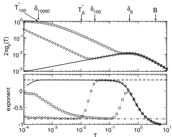
FIG. 21 Upper panel: g_p(T) for U = 0.5 , N = 10^4 , V_{l/r} = 10 , n = 1/2 , and N = 6 (squares), 100 (diamonds). The arrows indicate the relevant energy scales B , \delta_{N_D} , T_{N_D}^* and \delta_N . The solid curve shows g(T)/2 for a single barrier with V = 10 and U = 0.5 , N = 10^4 . Lower panel: Logarithmic derivative of the conductance. Dashed line: \gamma_o ; dashed-dotted line: \gamma_o/2 - 1 . (Data taken from Enss et al. (2005).)
