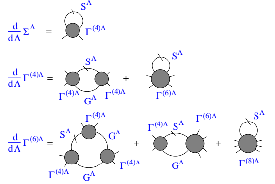
FIG. 3 (Color online) Diagrammatic representation of the flow equations for the self-energy \Sigma^\Lambda , the two-particle vertex \Gamma^{(4)\Lambda} , and the three-particle vertex \Gamma^{(6)\Lambda} in the one-particle irreducible version of the functional RG. Lines with a dash correspond to the single scale propagator S^\Lambda , the other lines to the full propagator G^\Lambda .
