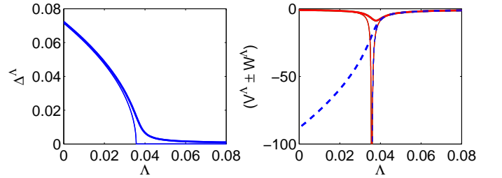
FIG. 14 (Color online) Flow for a reduced BCS model with a constant density of states at zero temperature; the band width is one and the bare interaction V = -0.3 . Left: Flow of the gap \Delta^\Lambda ; the thick line is for a bare gap \Delta_0 = 2.4 \cdot 10^{-4} and the thin line for \Delta_0 = 6 \cdot 10^{-8} , in units of the band width. Right: Flow of the linear combinations V^\Lambda + W^\Lambda (solid lines) and V^\Lambda - W^\Lambda (dashed lines) of normal and anomalous vertices. Thick lines are again for \Delta_0 = 2.4 \cdot 10^{-4} and thin lines for \Delta_0 = 6 \cdot 10^{-8} .
