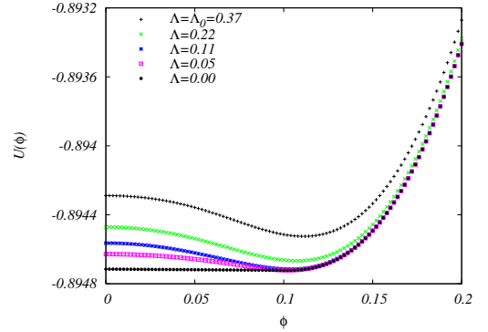
FIG. 15 (Color online) Flowing effective potential U_{\text{loc}}^{\Lambda}(\phi) for various values of \Lambda between \Lambda_0 = e^{-1} and 0, at \mu = -0.78 and T = 0.05 (Jakubczyk et al. , 2009).
