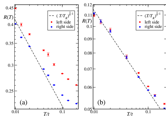
FIG. 2: (Color online) Effective backscattering amplitude R(T) on a logarithmic scale extracted from the amplitude of the density oscillations in Eq. (14) for a jump from (a) U_\ell = 0 to U_r = 1.8t , ( T_K = 3.4 \times 10^{-4}t ), and (b) U_\ell = 1t to U_r = 1.4t with t = t_\ell = t_r , ( T_K = 6 \times 10^{-6}t ). The amplitudes are extracted from fitting the local response for x < 0 (“left side”) and x > 0 (“right side”) separately.
