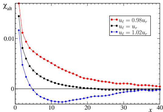
FIG. 3: (Color online) The alternating part of the density oscillations at T = 0.1t_r on the interacting side U = 1.8t_r , where the hopping on the non-interacting side is adjusted so that u_\ell = 0.98u_r , u_\ell = u_r , and u_\ell = 1.02u_r , respectively.
