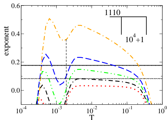
Figure 10. (Color online) System as in figure 8 with N_{\text{over}}^L = 1110 . Effective exponents in the regime v_F/N_{\text{over}}^L \ll T \ll B for different interaction strengths U . From bottom to top: U = 0.25; 0.5; 0.75; 1.0; 1.5 . The horizontal lines show the fRG approximation for \alpha_{\text{end}}(U = 0.5)/2 and \alpha_{\text{end}}(U = 1.0)/2 as obtained in [11]. The vertical line indicates the crossover scale.
