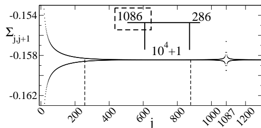
Figure 6. Off-diagonal self-energy at the end of the fRG flow for an interacting wire with U = 0.5 and couplings t^{cR} = t^{cL} = 0.25 at T = 4 \cdot 10^{-3} . The wire of length N = 10^4 + 1 is coupled to the end of the leads (i.e. N_{\text{lead}}^L = N_{\text{lead}}^R = 0 ) with N_{\text{over}}^L = 1086 , N_{\text{over}}^R = 286 . The part shown in the main plot is indicated by the dashed box in the inset. Long-ranged oscillations emerge from the boundaries and from the coupling site. The scale jT beyond which the oscillations are damped exponentially is indicated by the vertical dashed lines.
