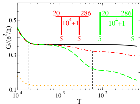
Figure 12. (Color online) As in figure 11 but with length N_{\text{mid}} = 10^4 + 1 and width N_{\text{con}}^L = N_{\text{con}}^R = 5 of contact region. Dashed-dotted line: N_{\text{lead}}^L = 0 , N_{\text{lead}}^R = 0 and N_{\text{over}}^L = 20 , N_{\text{over}}^R = 286 (setup shown in left inset). Dashed line: N_{\text{lead}}^L = 20 , N_{\text{lead}}^R = 286 and N_{\text{over}}^L = N_{\text{over}}^R = 0 (setup shown in right inset). Solid line: N_{\text{lead}}^L = N_{\text{lead}}^R = 0 and N_{\text{over}}^L = N_{\text{over}}^R = 0 . Dotted line: N_{\text{con}}^L = N_{\text{con}}^R = 1 , N_{\text{lead}}^L = N_{\text{lead}}^R = 0 and N_{\text{over}}^L = N_{\text{over}}^R = 0 for comparison. The vertical lines indicate the crossover scales.
