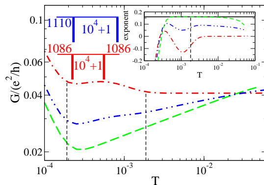
Figure 16. (Color online) As in figure 14 but with different N_{\text{over}}^L = N_{\text{over}}^R . Dashed line: N_{\text{over}}^L = N_{\text{over}}^R = 0 . Dashed-dotted line: N_{\text{over}}^L = N_{\text{over}}^R = 1086 . Dash-dot-dotted line: N_{\text{over}}^L = 1110, N_{\text{over}}^R = 0 .
