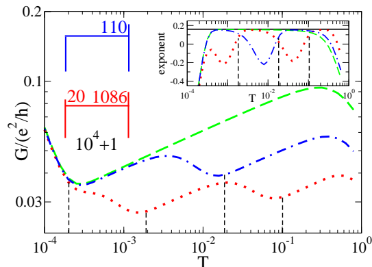
Figure 7. (Color online) Main plot: Conductance G of an interacting wire with U = 0.5 of length N = 10^4 + 1 as function of the temperature T . The coupling to the leads is located at the end of the wire ( N_{\text{over}}^L = N_{\text{over}}^R = 0 ) and has a small amplitude t^{cR} = t^{cL} = 0.25 . Dashed line: N_{\text{lead}}^{L/R} = 0 . Dashed-dotted line: N_{\text{lead}}^L = 0, N_{\text{lead}}^R = 110 . Dotted line: N_{\text{lead}}^L = 20, N_{\text{lead}}^R = 1086 . The vertical dashed lines terminating at the different curves indicate the corresponding crossover scales. Left inset: Setups studied. Right inset: Effective exponents. The solid horizontal line indicates the fRG approximation for \alpha_{\text{end}} as obtained in [11].
