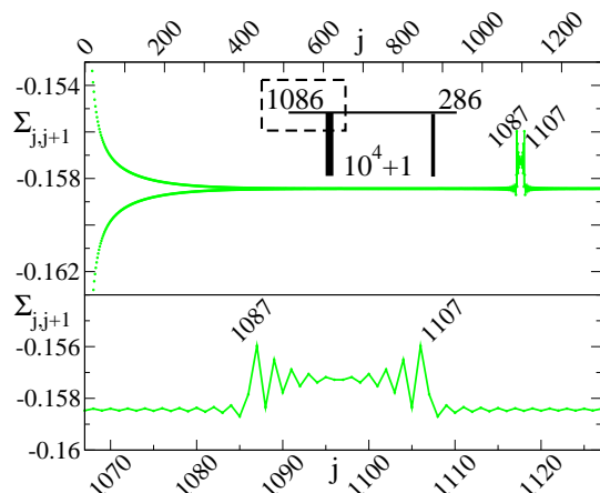
Figure 13. (Color online) Off-diagonal self-energy at the end of the fRG flow for an interacting wire with U = 0.5 at T = 4 \cdot 10^{-3} . All wire-lead couplings are set equal: t^{cR} = t^{cL} = 0.25 . The setup is shown in the inset: N_{\text{con}}^L = 5 , N_{\text{con}}^R = 1 , N_{\text{mid}} = 10^4 + 1 , N_{\text{lead}}^L = N_{\text{lead}}^R = 0 and N_{\text{over}}^L = 1086 , N_{\text{over}}^R = 286 . The part shown in the upper plot is indicated by the dashed box in the inset. Long-ranged oscillations emerge from the boundaries and from all coupling sites. The lower plot is a magnification of the left contact region.
