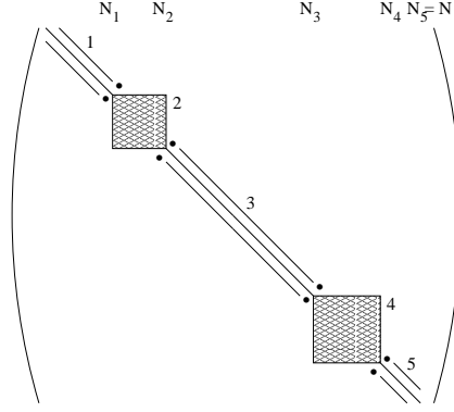
Figure A1. Structure of the inverse Green function for stripe-like leads: block 1,3 and 5 are tridiagonal (left, right overhang and middle part of wire), block 2 and 4 are full matrices (left and right contact region), the dots represent the connecting elements; (N_j, N_j) is the lower right element of the j -th block
