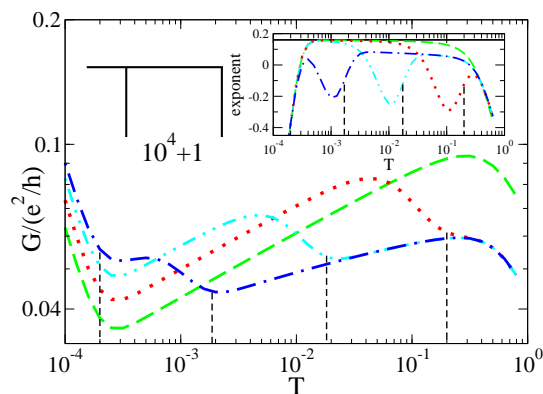
Figure 8. (Color online) As in figure 7 but with N_{\text{lead}}^L = N_{\text{lead}}^R = 0 , N_{\text{over}}^R = 0 and for different N_{\text{over}}^L . Dashed line: N_{\text{over}}^L = 0 . Dotted line: N_{\text{over}}^L = 11 . Dashed-double-dotted line: N_{\text{over}}^L = 111 . Dashed-dotted line: N_{\text{over}}^L = 1111 .
