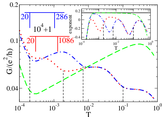
Figure 9. (Color online) The same as in figure 7 but with N_{\text{lead}}^L = N_{\text{lead}}^R = 0 and coupling into the bulk. Dashed line: N_{\text{over}}^{L/R} = 0 . Dashed-dotted line: N_{\text{over}}^L = 20, N_{\text{over}}^R = 286 . Dotted line: N_{\text{over}}^L = 20, N_{\text{over}}^R = 1086 .
