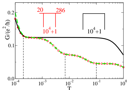
Figure 4. (Color online) Conductance G as function of temperature T of a noninteracting wire of length N = 10^4 + 1 and coupling t^{cR} = t^{cL} = 0.25 . Solid line: end-contacted wire, i.e. N_{\text{over}}^{L/R} = 0 (setup shown as the right inset) obtained from (14). Circles: N_{\text{over}}^L = 20, N_{\text{over}}^R = 286 (setup shown as the left inset) obtained from (14). Dashed line: the same parameters as for the circles but using the approximate analytical result (17). The vertical lines indicate the crossover scales resulting from the overhanging parts.
