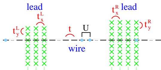
Figure 2. (Color online) Sketch of the 1d wire connected to stripe-like leads; the crosses depict the sites of the leads, the bars those of the wire; note that the coupling between the wire and the leads is located at arbitrary positions leading to overhanging parts.
