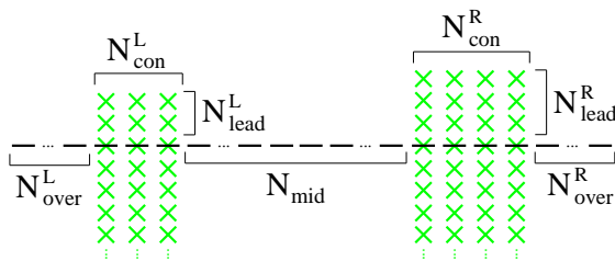
Figure 3. (Color online) Sketch of the system considered. The overlapping sites of wire and leads are individually coupled via a hopping term. The length scales are indicated.
