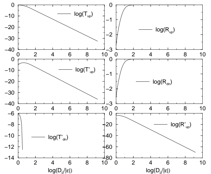
FIG. 5: Logarithm of transmission/reflection coefficients versus \log(D_0/|\epsilon|) . We may identify temperature T with |\epsilon| . Parameters are: g_\uparrow = 1 , g_\downarrow = 0.9 , g_\perp = 1.3 and v_{F-}/v_{F+} = 0.8 . For the initial noninteracting scattering amplitudes we used V = 0 , v_{F+} = 1 , \lambda = 0.05 .
