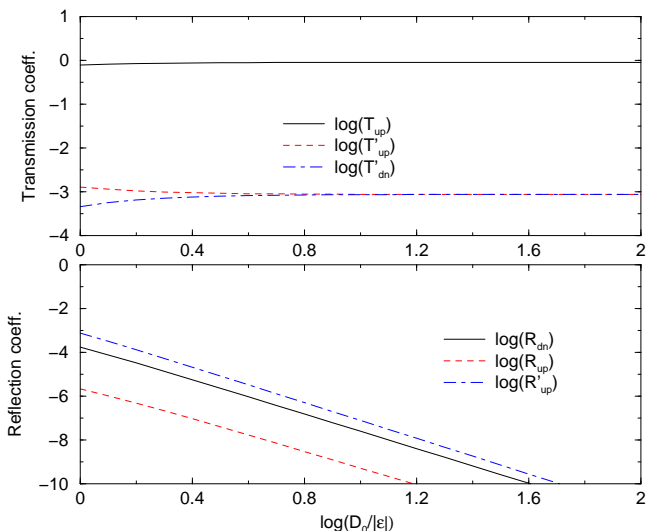
FIG. 6: Logarithm of transmission/reflection coefficients versus \log(D_0/|\epsilon|) . Parameters are: g_\uparrow = -0.7 , g_\downarrow = -1.1 , g_\perp = -1 and v_{F-}/v_{F+} = 0.8 . For the initial noninteracting scattering amplitudes we used V = 0 , v_{F+} = 1 , \lambda = 0.2 . The transmission coefficients are all finite as T \rightarrow 0 .
