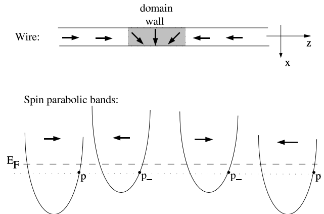
FIG. 1: Schematic of a domain wall and the relevant electron spin bands. States \psi_{p\uparrow} and \psi_{p-\downarrow} have the same energy.
